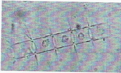
Chaetoceros
