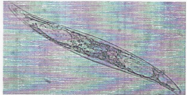
Gyrosigma
