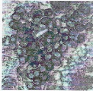
Microcystis
