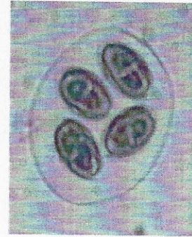
Oocystis
