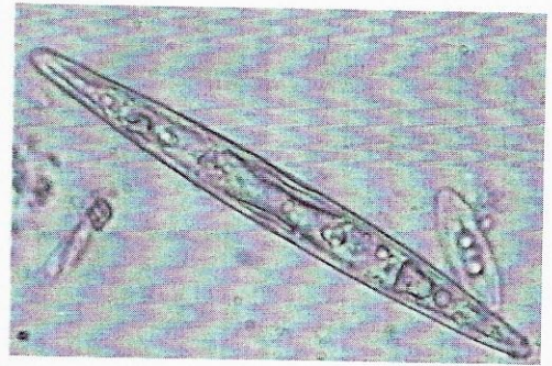
Pleurosigma
