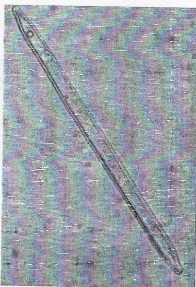
Syndra
