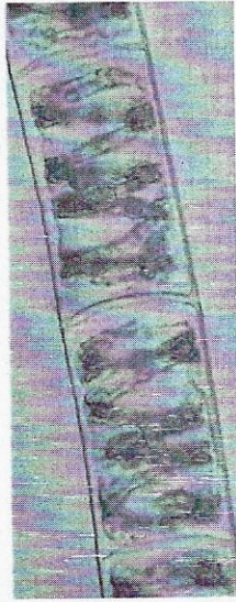
Spirogyra
