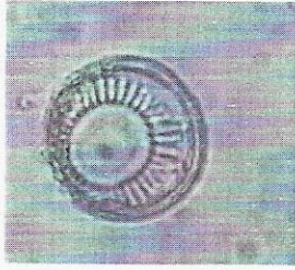
Cyclotella
