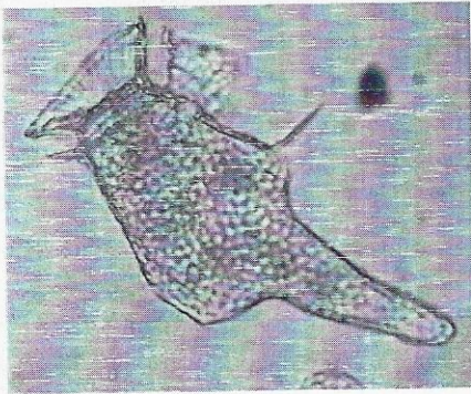
Dinophysis
