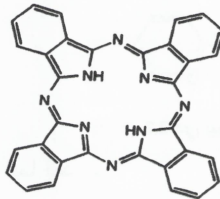
phthalocyanin
