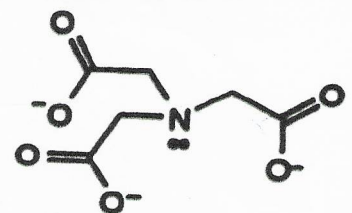
nitrilotriacetate NTA 3-
